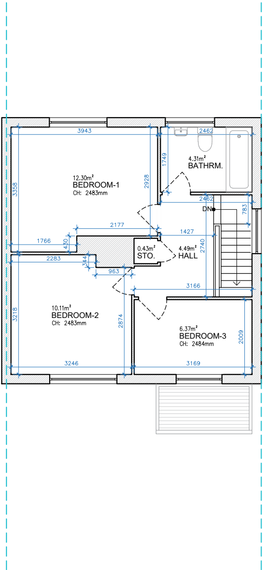
FIRST FLOOR GIA = 43.10 M 2
